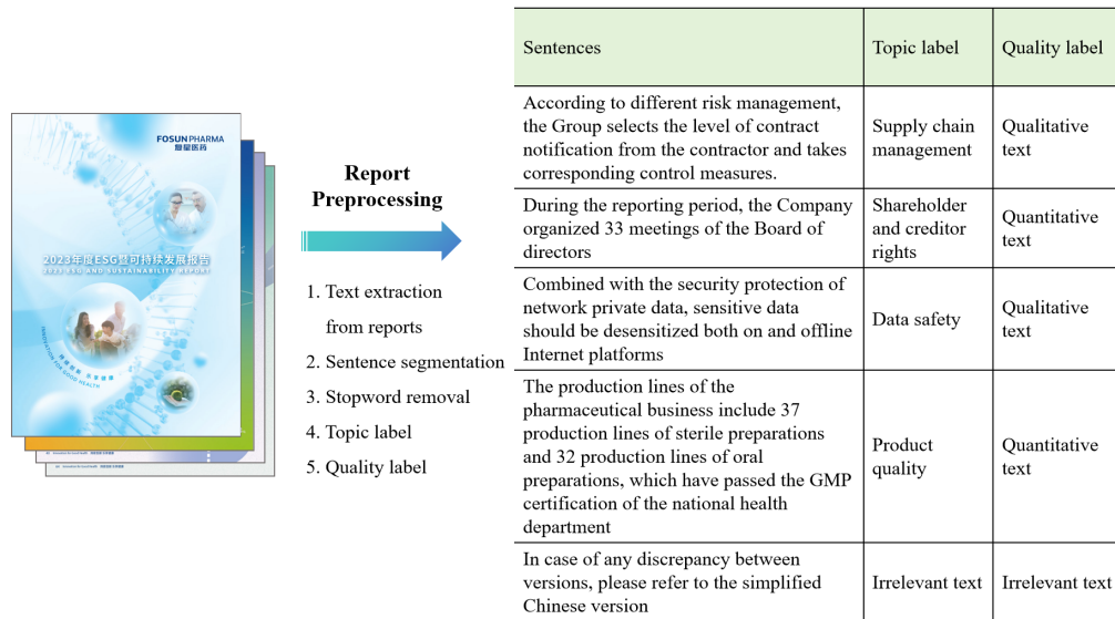
Figure 1: This image illustrates the preprocessing steps for an ESG report from stock 600196.
