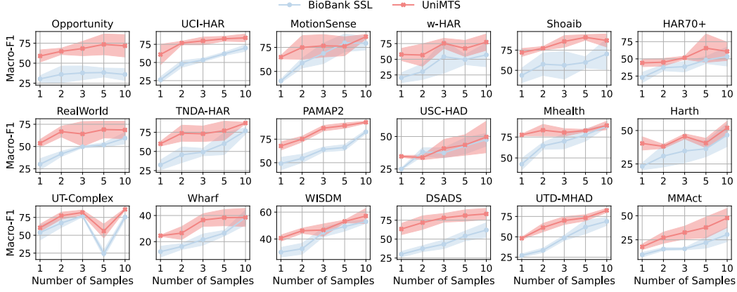
Figure 1: Few-shot fine-tuning results. UniMTS consistently outperforms BioBank SSL (Yuan et al. 2024). We repeat 3 runs and report both mean and standard deviation.
