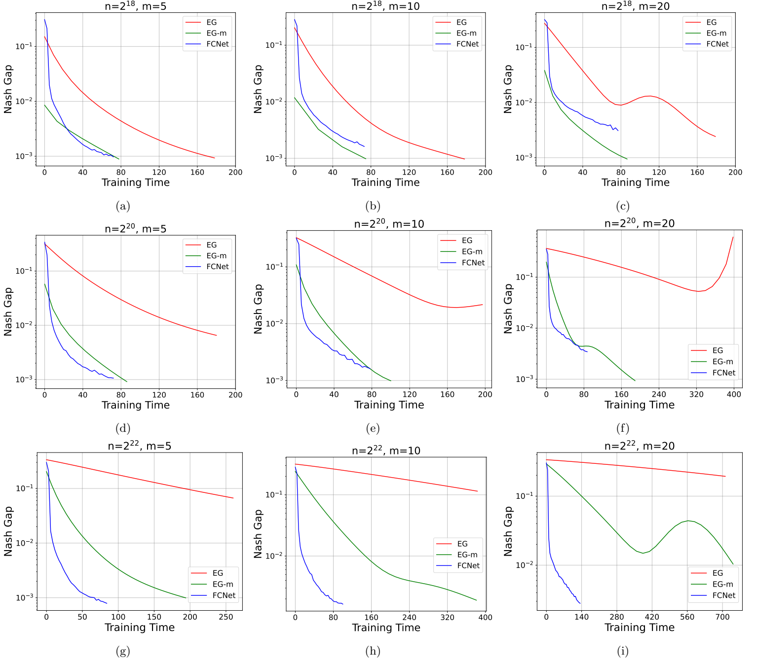
Figure 1: We provide the loss curve of MarketFCNet, EG and EG-m, corresponding to the experiments in Figure 3 in the original paper. The horizontal axis is the running time of MarketFCNet and baselines, and the vertical axis is the Nash Gap. Note that the Nash Gap coordinate is drawn in logarithm scale for better visualization. Recall that all methods are run with 30 epochs. EG and EG-m are early stopped when Nash Gap is less than 10^{-3} .
