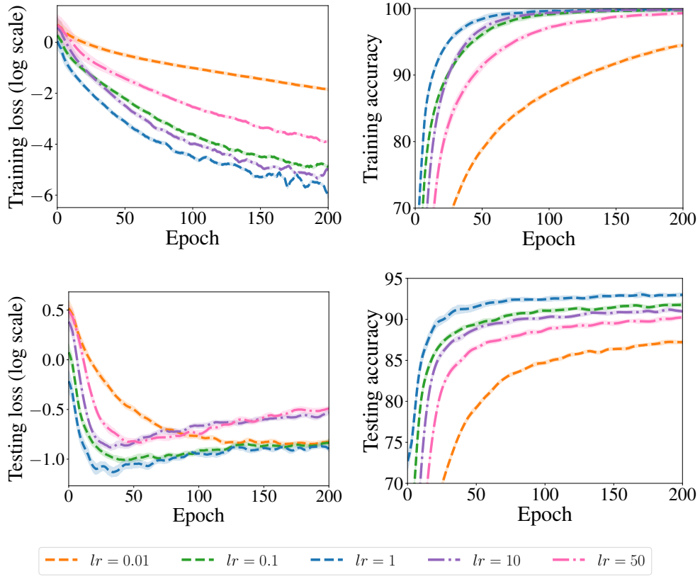
Figure 1: Results of STORM on the CIFAR-10 dataset with different learning rates.
