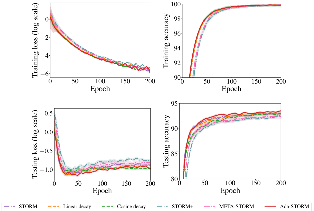
Figure 2: Results of different methods on the CIFAR-10 dataset.
