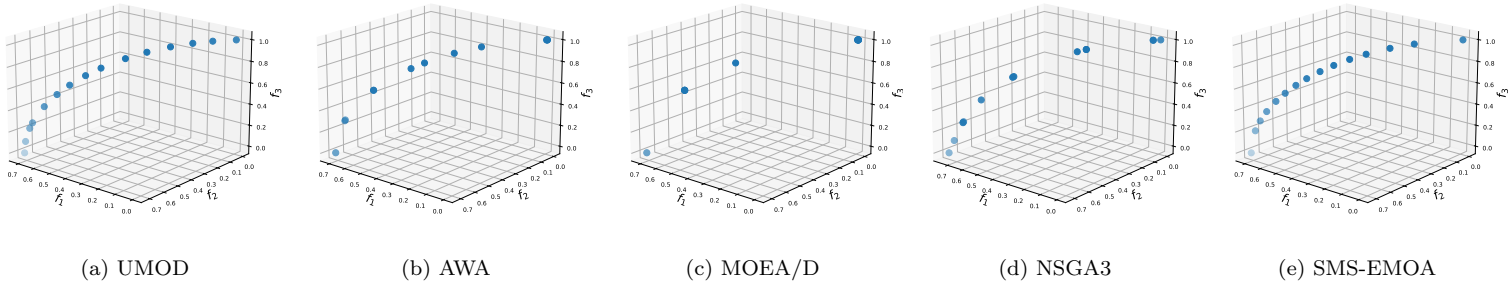
Figure 3: Comparison of using different methods on DTLZ5.
