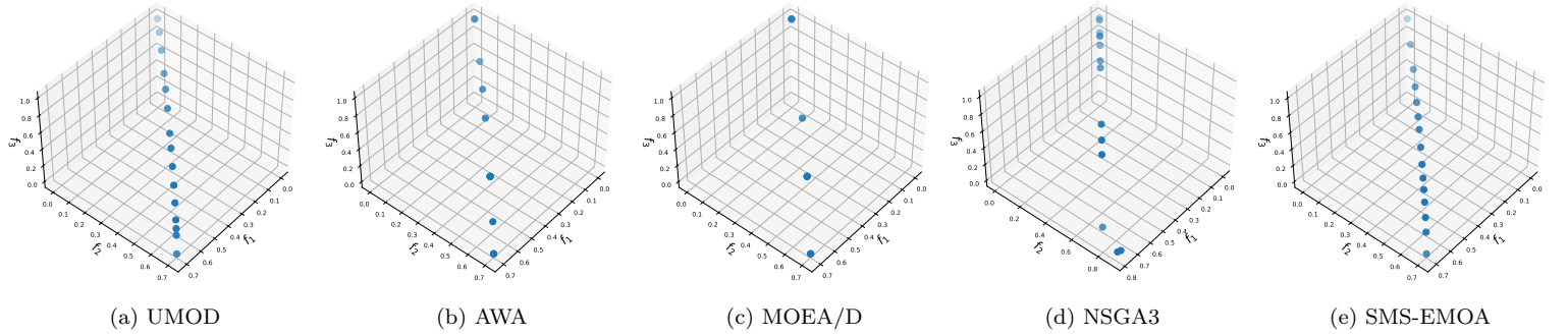
Figure 4: Comparison of using different methods on DTLZ6.
