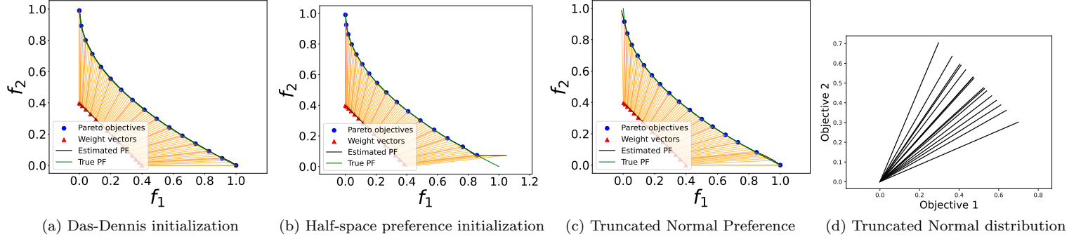
Figure 2: Comparison of using different initialization.
