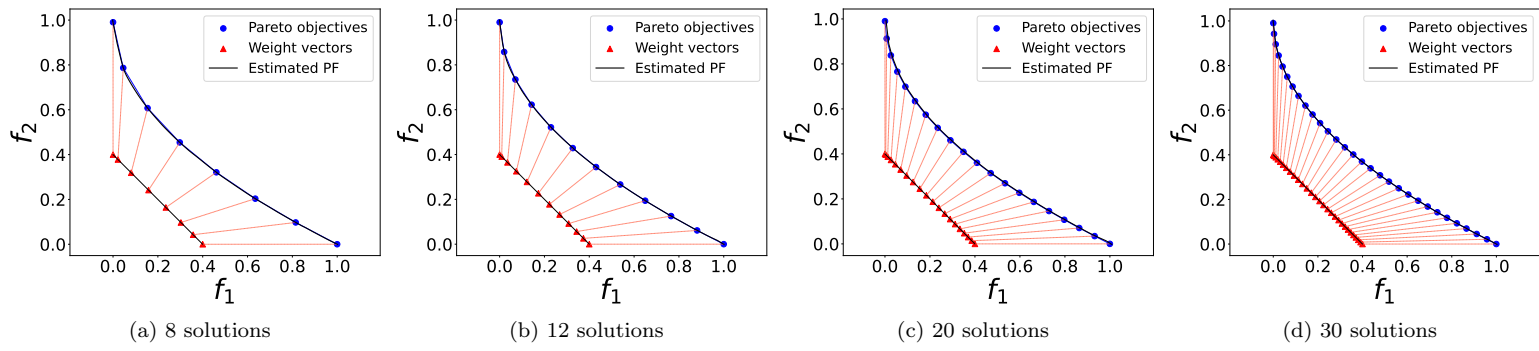
Figure 1: Results of using different number of K.
