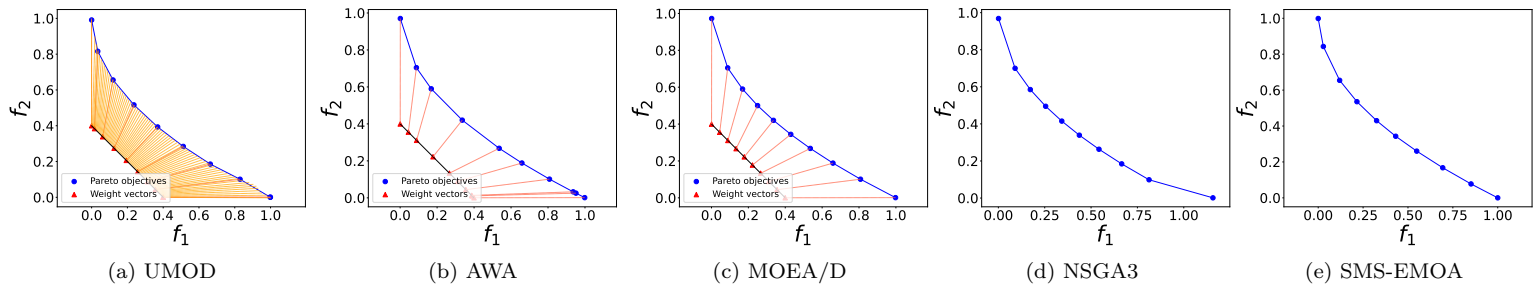
Figure 5: Results on F1.
