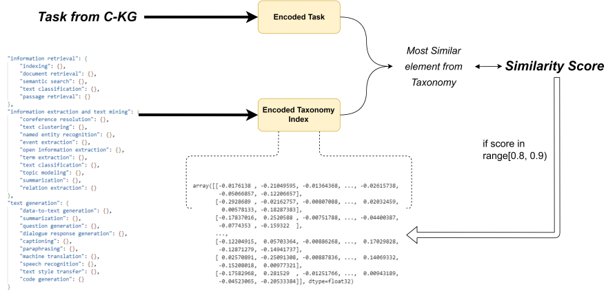
Figure 5: Taxonomy extension protocol: enriching a seed taxonomy with tasks from the C-KG.
