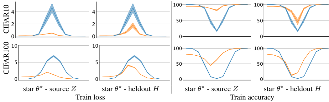
Figure 9: Loss barriers for DenseNet-40-12 star models on CIFAR. We plot training loss and accuracy curves obtained upon interpolation between star-regular and regular-regular models pairs. Star-regular loss barriers continue to be lower than regular-regular barriers, as observed in Figure 2.
