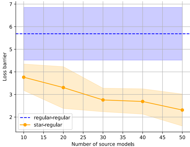
Figure 6: Transformer results. Star-regular barrier steadily decreases as we use more source models to train the star model.
