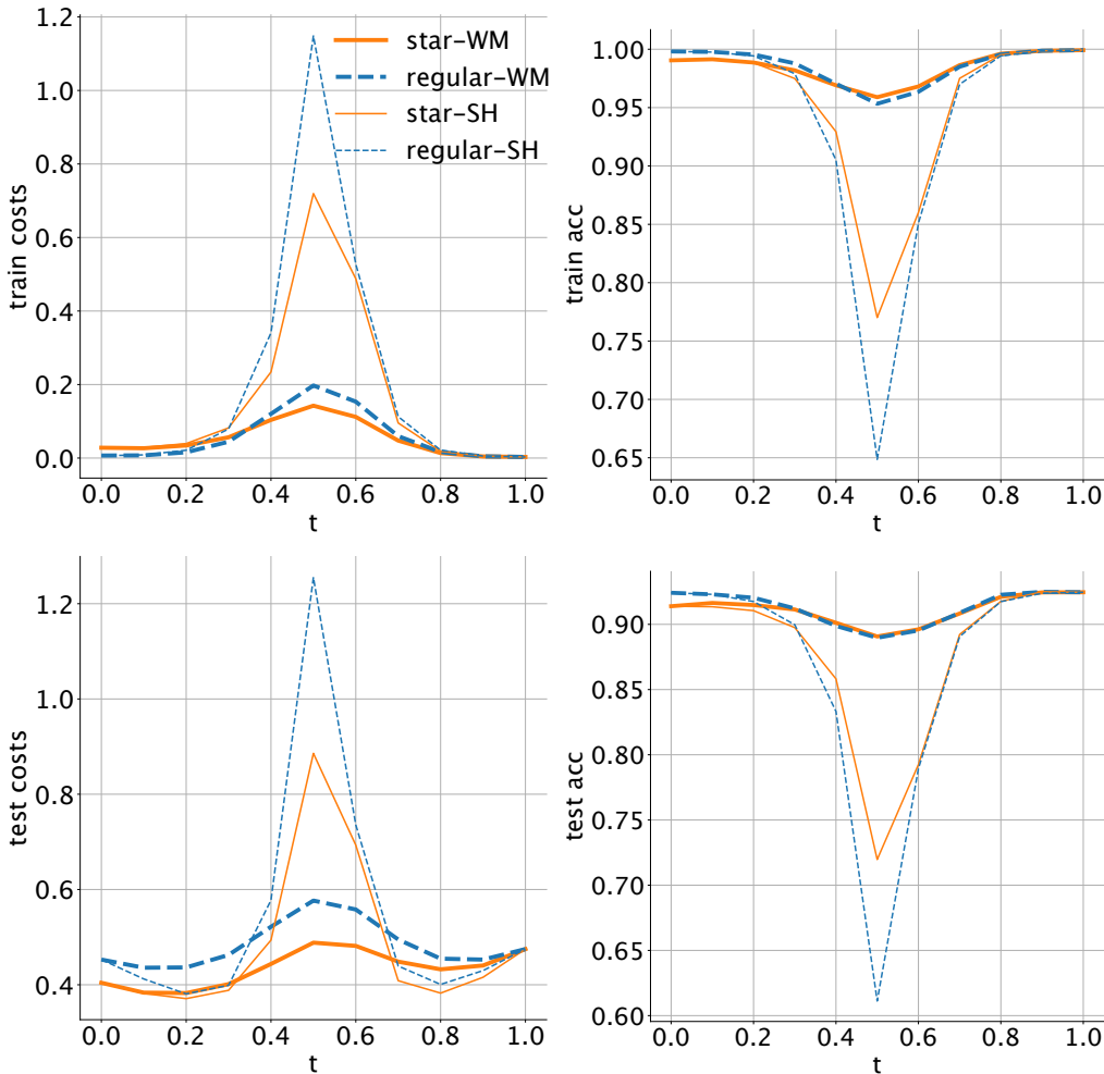
Figure 8: Effect of using Sinkhorn-rebasin instead of weight matching. We compare “star-regular” barriers against “regular-regular” barriers after fixing the permutation algorithm used to match the weights of the two models being interpolated. star-WM and regular-WM refer to the barriers after applying weight matching Ainsworth et al. (2022). Similarly, star-SH and regular-SH refer to barriers after applying Sinkhorn-rebasin Guerrero Peña et al. (2023). While vanilla WM outperforms SH in this case, a better hyperparameter choice may eventually cause SH to outperform WM. Nevertheless, the findings in this investigation further support our conclusion that star models are well-connected to other regular models, in comparison to how well the regular models are connected amongst themselves.
