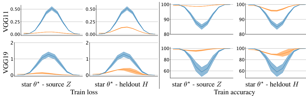
Figure 10: Loss barriers for VGG star models trained on CIFAR-10. Training loss and accuracy curves obtained upon interpolation between star-regular and regular-regular model pairs. We observe the same trend as in Figure 2.
