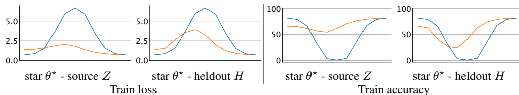
Figure 11: Loss barriers for ResNet18 star models trained on ImageNet-1k: training loss and accuracy curves obtained upon interpolation between star-regular and regular-regular model pairs. While ImageNet models struggle to achieve LMC, star-regular barriers still fare much better than regular-regular barriers.
