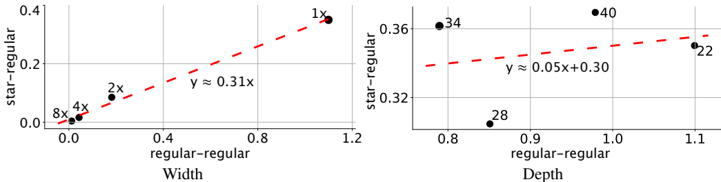
Figure 3: “Starness” vs. model width and depth. For starness vs. model width (left), we vary the width of a WideResNet (depth 22) from 1\times to 8\times . For starness vs. model depth, we vary the depth of a WideResNet (width 1\times ) from 22 to 40 layers. For each depth-width combination, we plot the loss barriers B(\theta^*, \theta_h) between star models \theta^* and heldout models \theta_h \in H on the y-axis. As a reference point, we plot the barrier between two regular solutions B(\theta_A, \theta_B) , on the x-axis. The points are annotated with the corresponding widths or depths. Star models consistently enjoy better linear connections with regular models, than do the regular models amongst each other.
