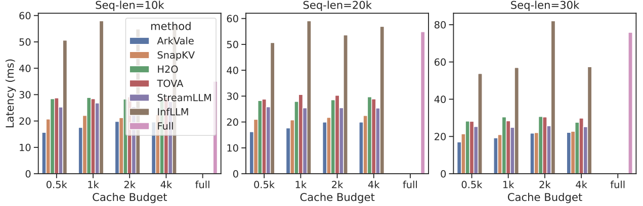
Figure 2: Per-step decoding latency of LongChat-7B-v1.5-32k with different methods, sequence-lengths, and cache-budgets.
