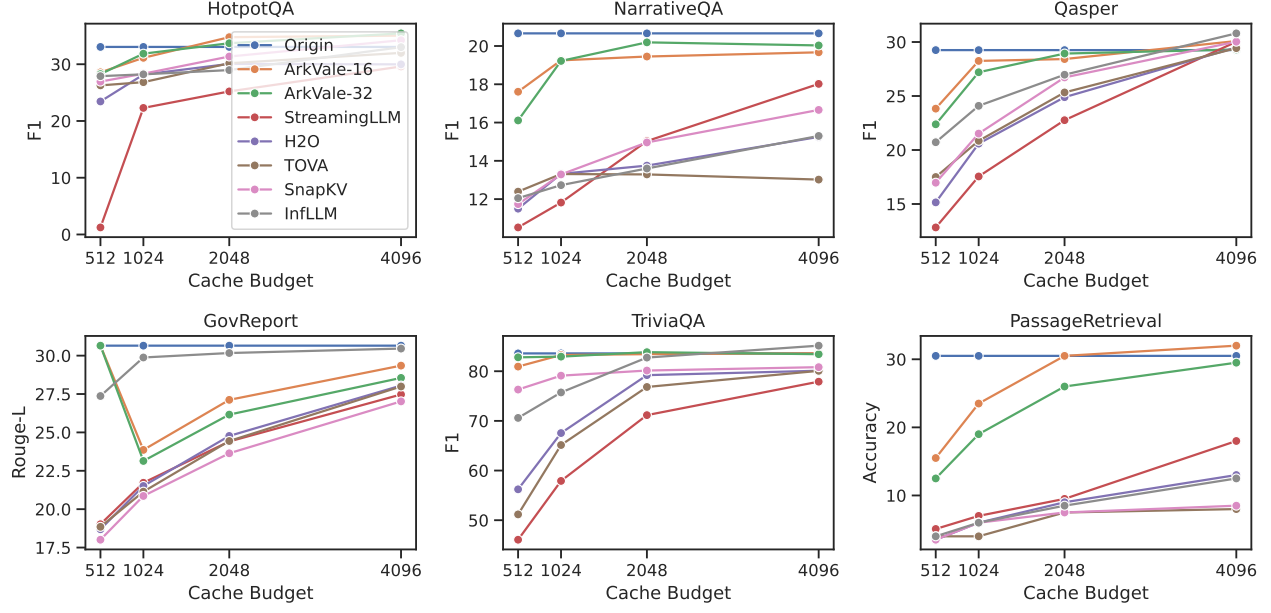
Figure 1: Evaluation of LongChat-7B-v1.5-32k on LongBench with different methods and cache-budgets.
