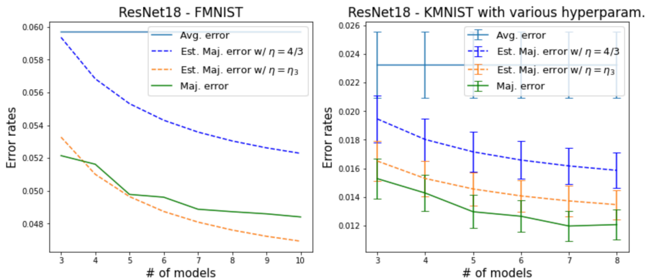
Figure C. Additional plots to Figure 3 with FMNIST, KMNIST
