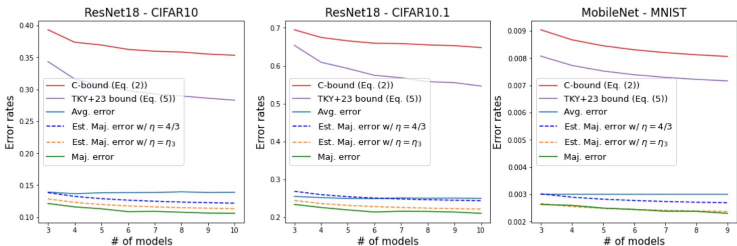
Figure B. Figure 3 with other bounds described in Section 2.2
