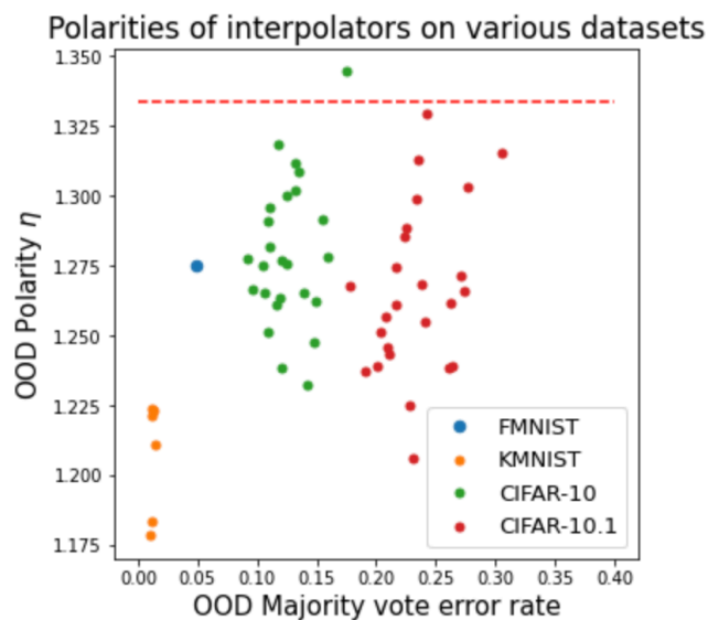
Figure A. Polarities of interpolators on various datasets
