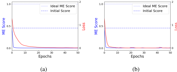
Figure 7: Results for the synthetic seq2seq task. The configurations shown in the setting are (a) Results for a seq2seq GRU without attention (b) Results for a seq2seq GRU with attention.
