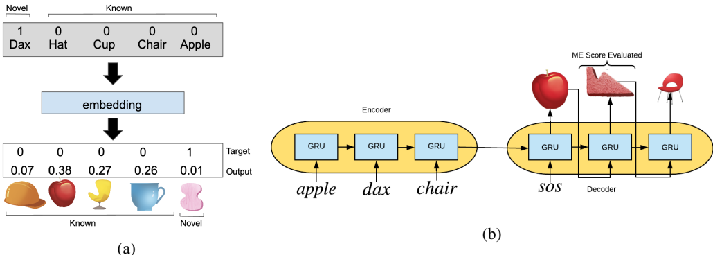
Figure 2: Evaluating mutual exclusivity in a feedforward (a) and seq2seq (b) neural network. (a) After training on a set of known objects, a novel label (“dax”) is presented as a one-hot input vector. The network maps this vector to a one-hot output vector representing the predicted referent, through an intermediate embedding layer and an optional hidden layer (not shown). A representative output vector produced by a trained network is shown, placing almost all of the probability mass on known outputs. (b) A similar setup for mapping sequences of labels to their referents. During the test phase a novel label “dax” is presented and the ME Score at that output position is computed.
