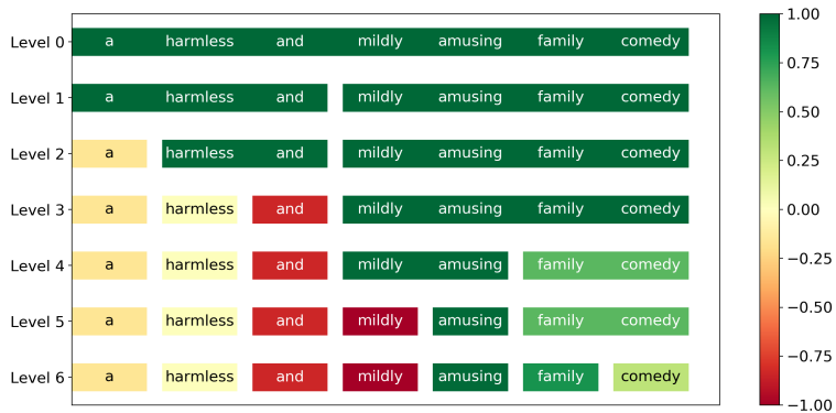
Figure 14: INTERSHAPLEY for BERT on a positive movie review from SST dataset, on which BERT makes correct prediction. Red and green colors represent the negative and positive sentiments respectively.
