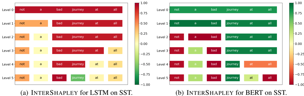
Figure 4: INTERSHAPLEY for LSTM and BERT on a positive movie review from SST dataset, on which BERT makes correct prediction (positive), while LSTM makes wrong prediction (negative). Red and green colors represent the negative and positive sentiments respectively.
