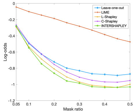
(b) Log-odds of BERT on SST dataset.
