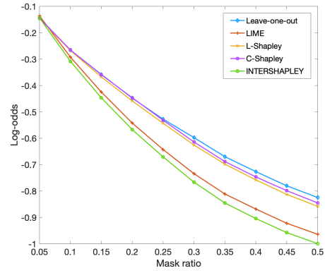
(b) Log-odds of CNN on SST dataset.
