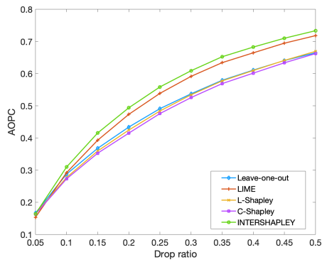
(a) AOPCs of CNN on SST dataset.
