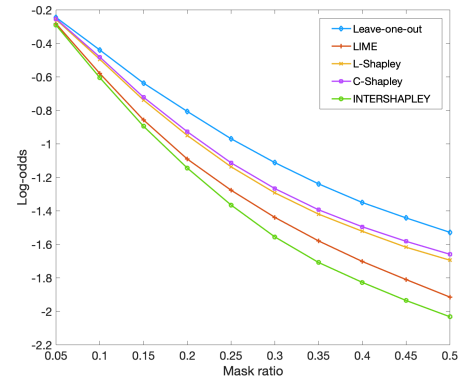
(b) Log-odds of CNN on IMDB dataset.
