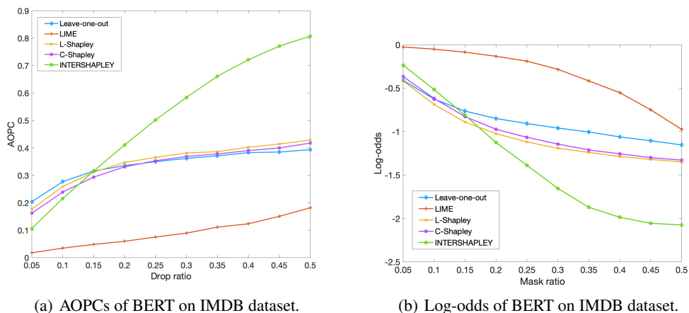
Figure 10: The AOPC and log-odds scores of BERT on IMDB dataset.
