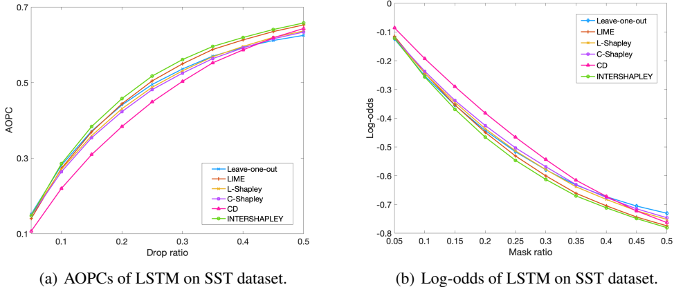
Figure 2: The AOPC and log-odds scores of LSTM on SST dataset.
