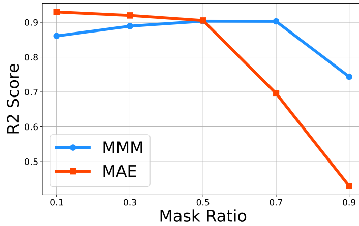
Figure 3: R2 score on the test samples of SEED
