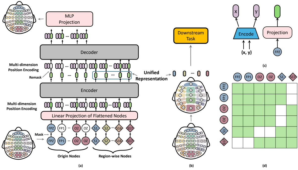
Figure 1: Revised overview of our methods
