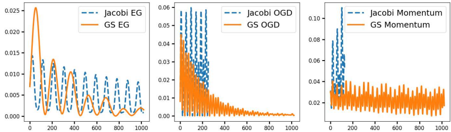
Figure 3: Jacobi vs. GS updates. y-axis: Squared distance \|\phi - v\|^2 . x-axis: Number of epochs. Left: EG with \gamma = 0.2, \alpha = 0.02 ; Middle: OGD with \alpha = 0.2, \beta_1 = 0.1, \beta_2 = 0 ; Right: Momentum with \alpha = 0.08, \beta = -0.1 . We plot only a few epochs for Jacobi if it does not converge.
