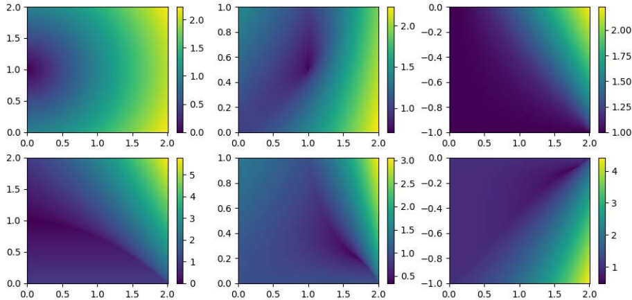
Figure 2: Heat maps of the spectral radii of different algorithms. We take \sigma = 1 for convenience. The x -axis is \alpha and the y -axis is \beta . Top row: Jacobi updates; Bottom row: Gauss-Seidel updates. Columns (left to right): EG; OGD; momentum. If the spectral radius is strictly less than one, it means that our algorithm converges. In each column, the Jacobi convergence region is contained in the GS convergence region (for EG we need an additional constraint, see Theorem 3.2).
