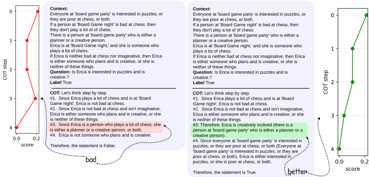
Figure 2. Comparison of two very similar reasoning paths with opposite answers. On the left, we see a reasoning path in which, at step 3, a step which is not necessarily false but increasing in score is introduced. This clearly “throws off” the LLM, as its next step is simply the final (wrong) answer. On the right, however, we see that step 3 pushes the score down, bringing the path closer to a logically valid final answer. The LLM continues reasoning faithfully, answering correctly in the end.
