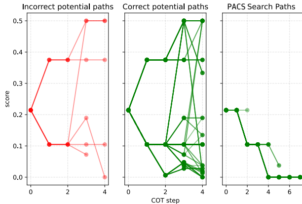
Figure 1. The (normalized) score progression of LLM sampled and PACS sampled paths. On the left and middle, we generate paths exhaustively taking 3 sample next-thoughts at each node. On the left, we show the model-count-based scores for incorrect paths and in the middle for the correct ones. We find no discernible difference between correct and incorrect score behaviour, indicating unfaithful LLM reasoning. On the right however, PACS shows that when using our minimization approach we find well-minimized paths which are all correct . This shows that the LLM itself can not properly solve the minimization we describe, and eventually gives up with a guess. This is validated by analysis of the text generated over the paths, shown in Figure 2.
