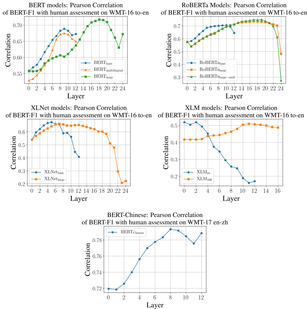
Figure 3: Pearson correlation of F_{\text{BERT}} computed with different models, across different layers, with segment-level human judgments on WMT16 to-English machine translation task. The WMT17 English-Chinese data is used for the BERT Chinese model. Layer 0 corresponds to using BPE embeddings. Consistently, correlation drops significantly in the final layers.
