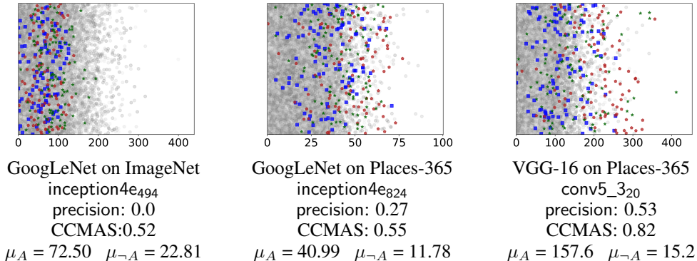
Figure 5: The units with with the highest Network Dissection scores for the category ‘bus’. The scatter plots, precision, and CCMAS scores all indicate a low selectivity for this category. blue squares: ‘school bus’; red pentagons: ‘trolleybus’; green stars: ‘minibus’; grey circles: other classes.
