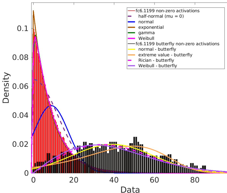
Figure 11: Fitting the non-zero activations for all classes (red) and the maximum activation class (black). For the superset of all the classes, the distribution is well-described by exponential-derived fits, normal-derived fits are bad. For the maximum activating class (butterfly), the distribution has a mean and can be well-described as a normal distribution.
