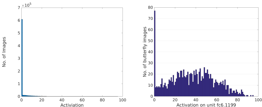
Figure 10: The distribution of activations on unit fc6.1199 for all images (left). 82.8% of activations are zero across all classes, only 5.8% of the butterfly class are zero. Unit fc6.1199 is a butterfly detector under Zhou et al. (2015)’s precision measure. Bins are 1.0 wide.
