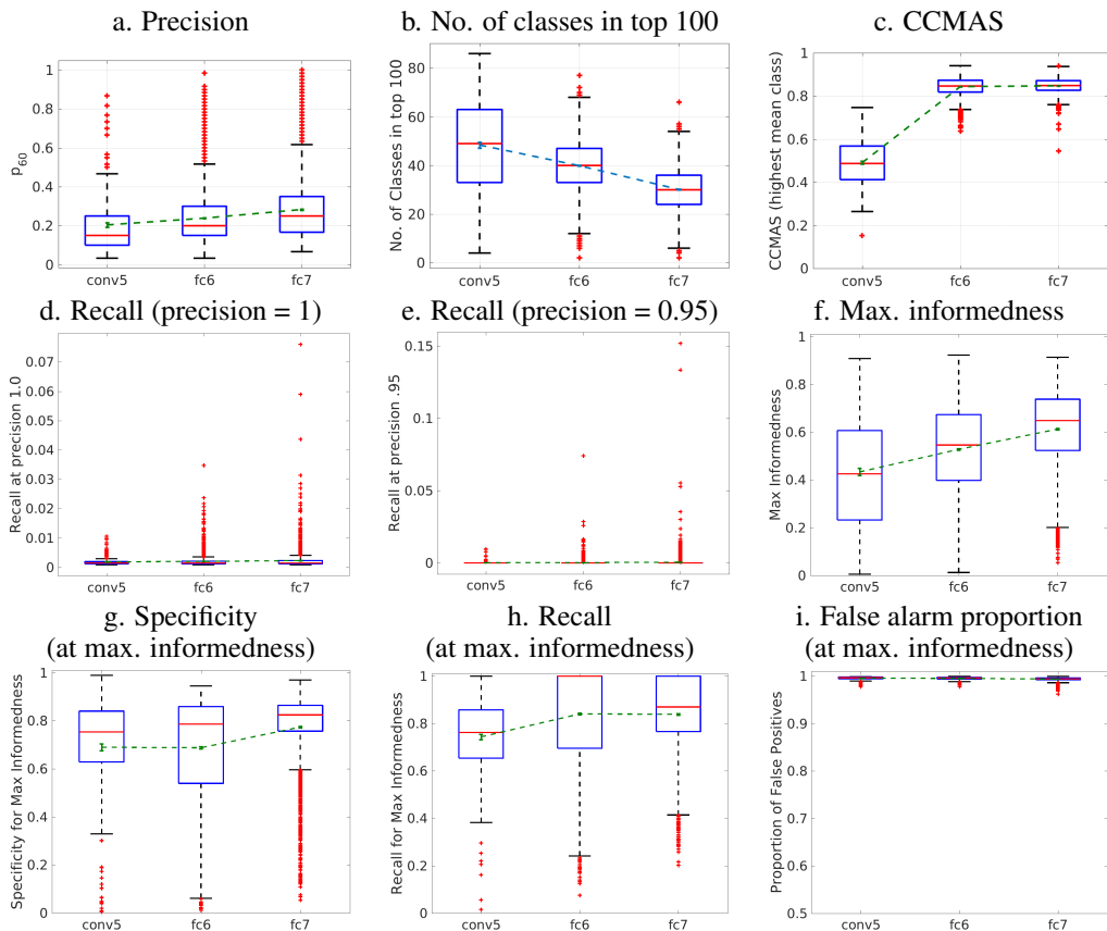
Figure 2: Different selectivity measures across the conv5, fc6, and fc7 layers of AlexNet. Red-line: median of data, top and bottom of box edges is the 25 th and 75 th percentile, whiskers extend to extreme edges of distribution not considered outliers and red crosses are outliers. Green points and dashed lines are the means of the distributions with standard errors. The high levels of selectivity observed with the precision and CCMAS measures are in stark contrast with the low levels of selectivity observed with the recall with perfect precision and high false-alarm rates at maximum informedness.
