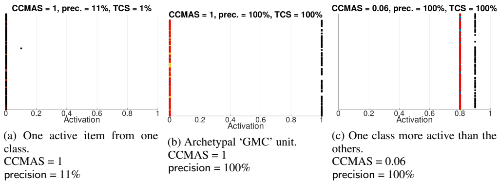
Figure 12: Example of where the CCMAS does not match intuitive understandings of selectivity. Generated example data: (a) If a unit is off to all but a single image from a large class of objects, the CCMAS for that class is 1 (maximum possible selectivity). (b) If a unit is strongly activated to all members of one class and off to everything else (an archetypal ‘grandmother’ cell) the CCMAS is the same as for (a) although the precision is vastly different. (c): If a unit has high activations for all classes, but one class (black squares) is 0.1 more than all others (coloured circles), the CCMAS is very low (0.06) despite being %100 precision. The generated examples are for 10 classes of 100 items
