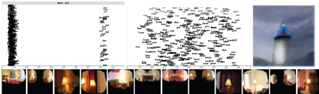
Figure 1: Examples of selectivity measures used. Top left: jitterplot of unit 113 in an RNN (under the superposition constraint) selective to the letter ‘j’ (Bowers et al., 2016). Top middle: jitterplot of a non-selective unit 160 found in an RNN trained on words one-at-a-time from (Bowers et al., 2016). Top right: Activation maximization image of unit conv5 0 AlexNet that resembles a lighthouse (Nguyen et al., 2016). Bottom: highest-activation images for a ‘lamp’ detector with 84% precision in the layer conv5 of AlexNet; from (Zhou et al., 2015).
