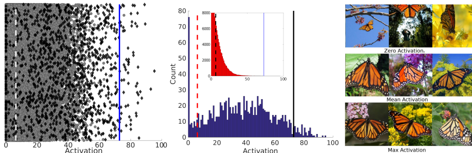
Figure 3: Data for unit fc6_{1199} . Left: activation jitterplot, black diamonds: Monarch butterfly images; grey circles: all other classes; white dashed line: threshold for the butterfly class maximum informedness; blue solid line: threshold for top 60 activations. Middle: histogram of activations of Monarch butterflies. Inset: zoomed-in histogram of all activations across all ImageNet classes of unit fc6_{1199} (N.B. this plot shows only the highest 121,586 activations; there are 596,734 activations at 0). There are Monarch butterfly images covering the whole range of values, with 72 images (5.8% of the total) having an activation of 0. Right: example ImageNet images with activations of 0 (top), the mean, 39.2 \pm 0.6 , (middle), and the maximum, 95, (bottom) of the range. Although the high precision score suggests that this unit is a butterfly detector this is misleading given there are butterfly images over the entire activation range (including 0).
