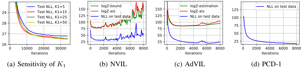
Figure 3: (a) Sensitivity analysis of K_1 on the Digits dataset. (b-d) Learning curves of NVIL, AdvIL and PCD on the Mushrooms dataset. Compared with NVIL, AdvIL provides a tighter and lower variance estimate of \log \mathcal{Z} and achieves better performance. Compared with PCD, AdvIL can track the log partition function and achieve comparable results though trained in a black-box manner.
