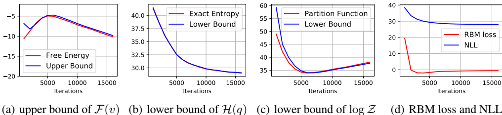
Figure 2: Results of AdvIL on the binary digits dataset. (a-c) compare the value of the variational approximations and the corresponding ground truths. All bounds are rather tight after 5,000 iterations. (d) shows that the RBM loss tends to zero and the model converges gradually.
