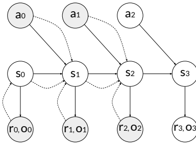
Figure 2: Probabilistic graphical model of the POMDP. The only variables observed (shaded nodes) are the actions, observations (high-dimensional images), and rewards. Our model has to infer the latent space (dashed lines) as well as to model the conditional probabilities (solid lines).
