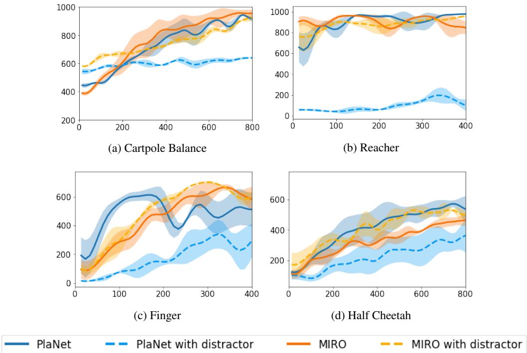
Figure 5: Learning curves of MIRO and PlaNet on environments with and without distractors. All curves represent mean and the shaded area represents one standard deviation among 3 seeds. MIRO’s performance remains unchanged in the presence of distractor objects in the environments while PlaNet is drastically affected by such objects. When no distractors are present in the scene both approaches have comparable performance.
