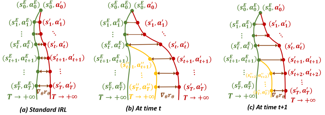
Figure 4: An illustration of how we consider the entire horizon.
