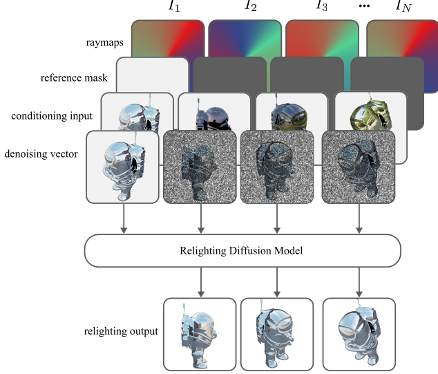
Figure 1. Relighting model overview. For each input image, we pass to the model raymaps containing the pose information, a binary mask to highlight which frame is being treated as the reference, and the conditioning images of the object under varying illumination. We concatenate all the inputs to the image being currently denoised. Note that both the conditioning inputs and target images are the latent encoding of the images, but we show them as images here for simplicity.
