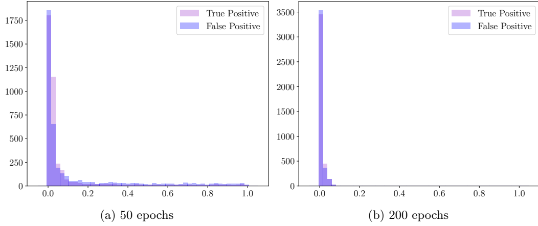
Figure S2: The normalized similarity distribution of true positive and false positive pairs of DIVIDE.
