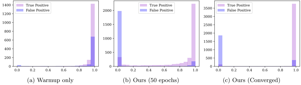
Figure S3: The normalized similarity distribution of true positive and false positive pairs of CANDY.
