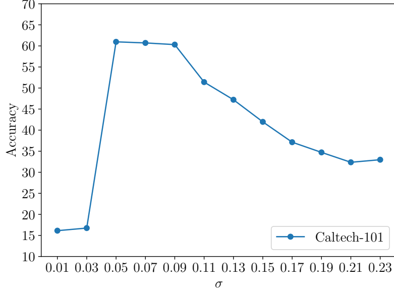
Figure S1: The influence of \sigma in the Gaussian kernel on Caltech-101 dataset.
