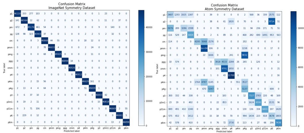
Figure 1: Confusion matrix of train and cross-validation accuracy with ResNet50 model.
