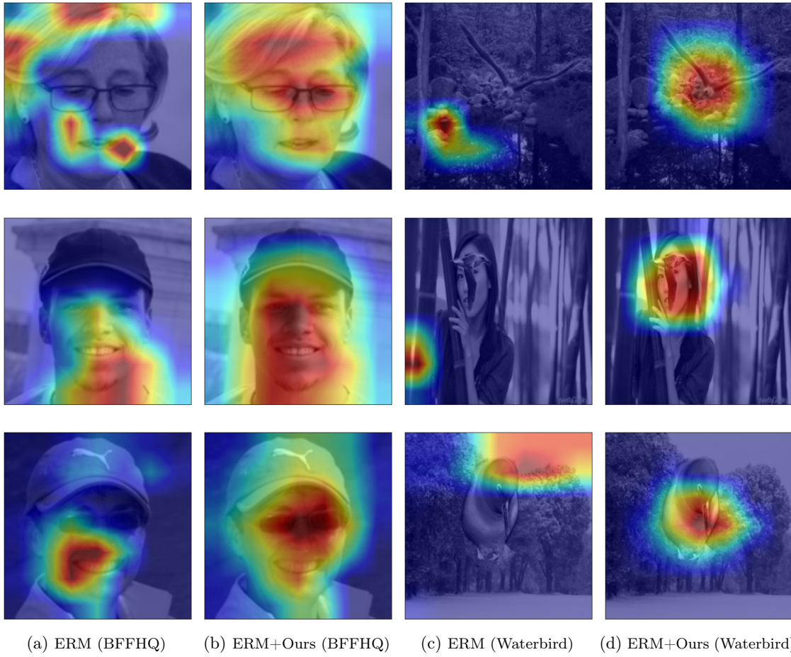
Figure 1: The Grad-CAM of ERM and ERM+Ours on BFFHQ and Waterbird. (a) and (c) denote Grad-CAM of ERM. (b) and (d) indicate Grad-CAM of ours combined with ERM.
