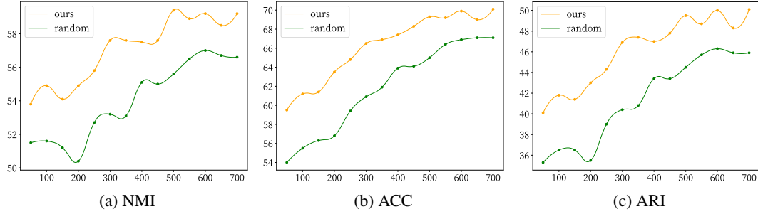
Figure 2: Influence of different numbers of selected samples M on CIFAR-20. NMI, ACC, and ARI curves are shown in (a), (b), and (c), respectively.
