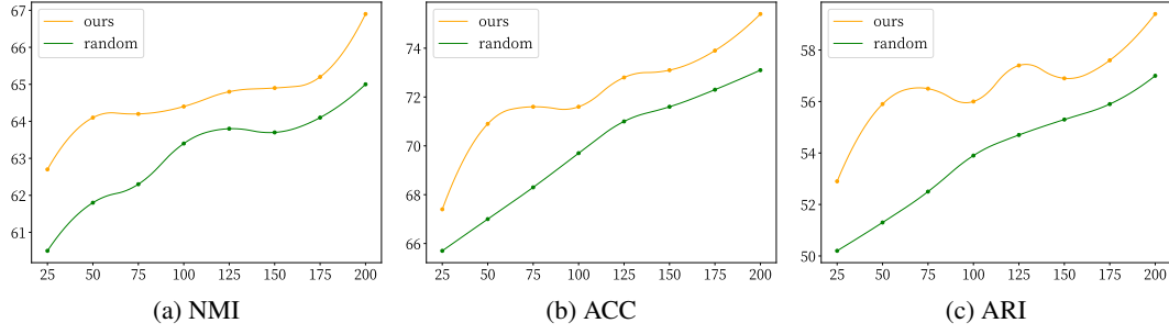
Figure 1: Influence of different numbers of selected samples M on ImageNet-Dogs. NMI, ACC, and ARI curves are shown in (a), (b), and (c), respectively.
