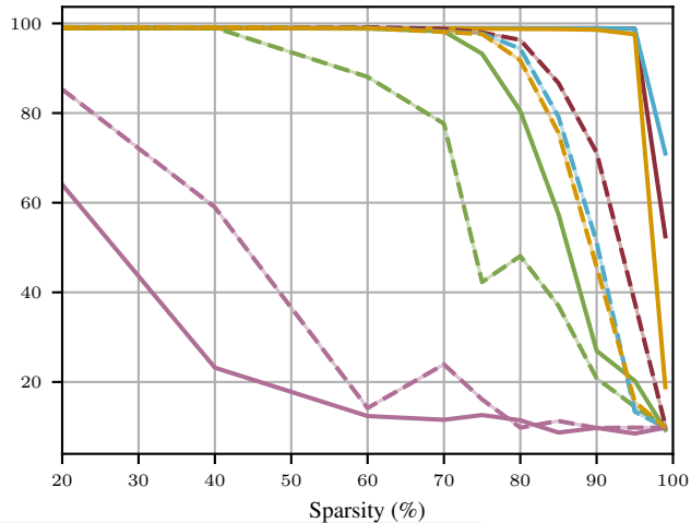
LeNet on MNIST
