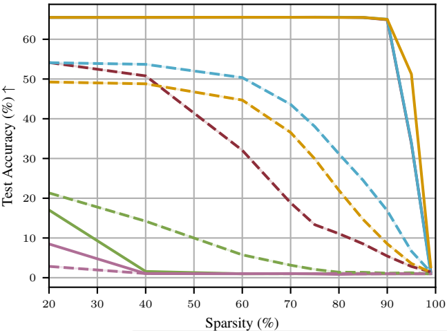
WRN on CIFAR-100
