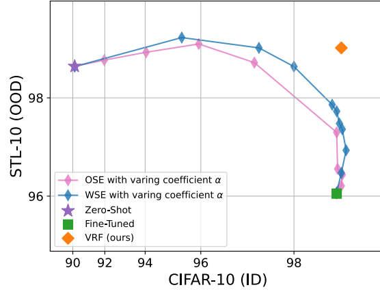
Figure 10: ID-OOD frontier curves for OSE and WSE for CIFAR-10 \rightarrow STL10.
