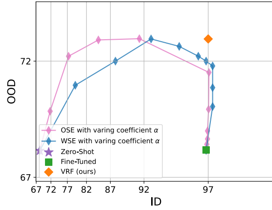
Figure 11: ID-OOD frontier curves for OSE and WSE for Entity-30.
