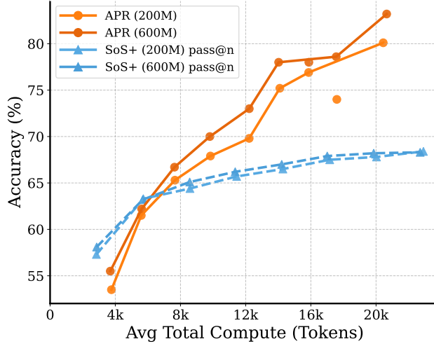
Figure 8: Accuracy vs. average total compute (in thousands of tokens) for 200M and 600M parameter models. APR consistently outperforms SoS+ and scales more strongly with model size.
