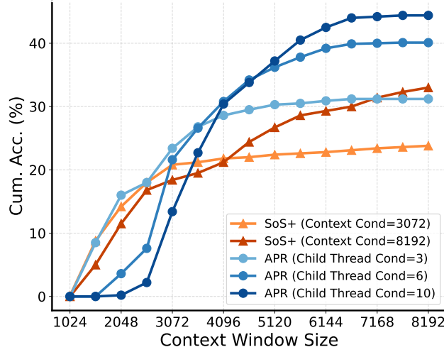
Figure 9: Accuracy vs. context window size on the five-number Countdown task for SoS+ and APR.
