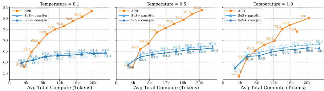
Figure 10: Ablation of APR and SoS+ vs. total compute under different temperature settings. Across all settings, APR demonstrates more reliable and efficient scaling behavior.
