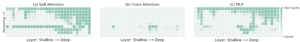
Figure 1: The learned router for PixArt-XL-2-512x512. The base solver is DPM-Solver with 20 NFEs.
