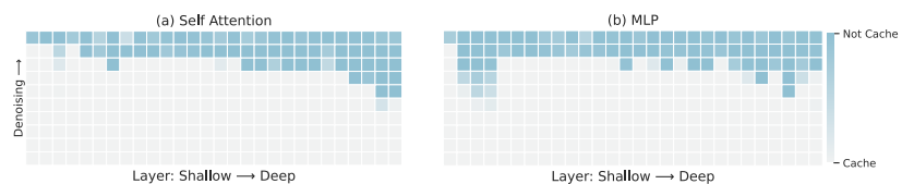
Figure 3: The learned router for DiT-XL-2. The base solver is DDIM with 20 NFEs.
