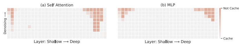
Figure 2: The learned router for U-ViT-H/2. The base solver is DPM-Solver with 20 NFEs.
