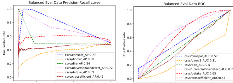
Figure 2: Precision-Recall curve with AP and AUC-ROC for each detector evaluated on a balanced Semi-Truths Eval Dataset
