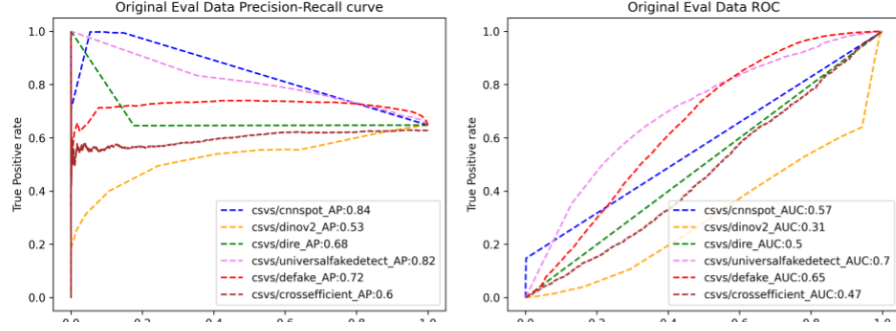
Figure 1: Precision-Recall curve with AP and AUC-ROC for each detector evaluated on Semi-Truths Eval Dataset
