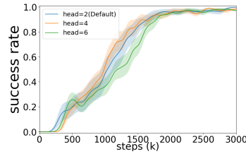
(b) Number of prediction heads
