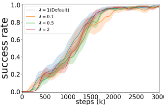
(a) Auxiliary loss weight \lambda
