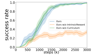
(c) Intrinsic reward & Curriculum
