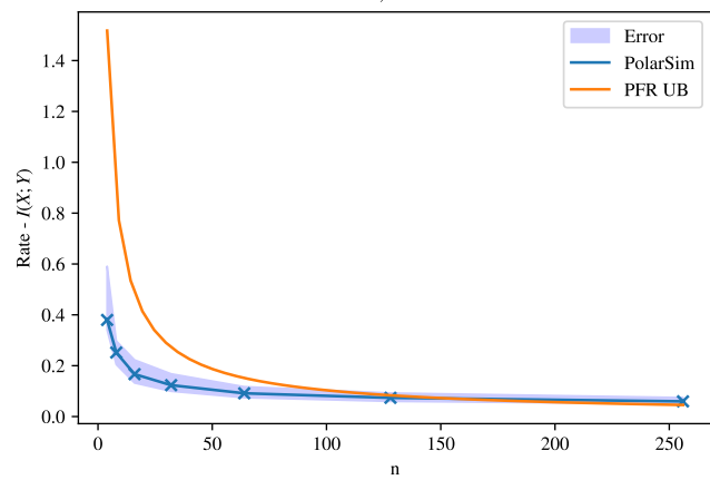
BEC, \varepsilon = 0.2
