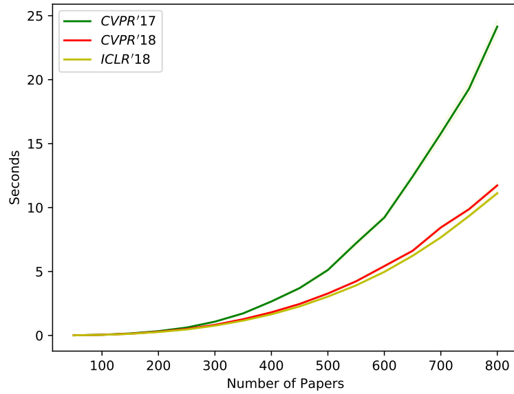
Figure 1: Running time of CoBRA as a function of the number of submissions to the conference. Submissions were subsampled from the three datasets shown in the legend. Results are averaged over 25 runs, shown together with the standard error.
