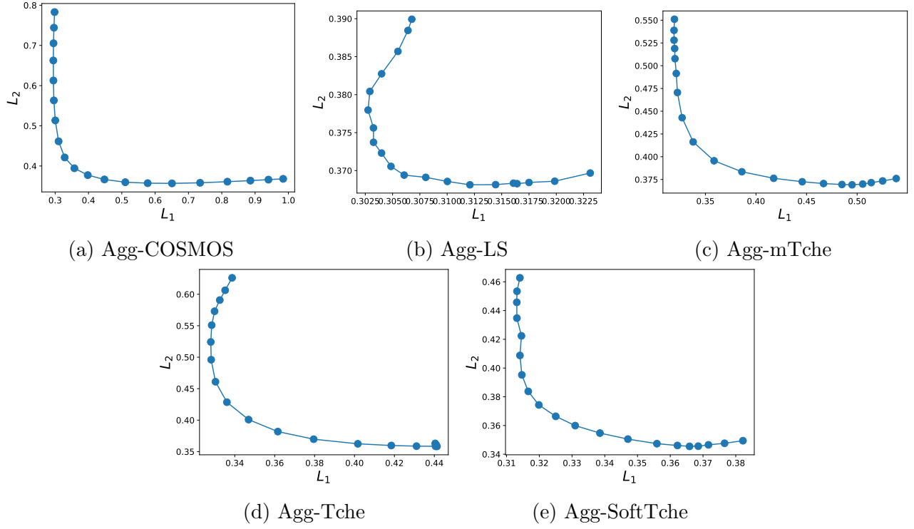
Figure 1: Predicted Pareto solutions from a Pareto neural model on MO-MNIST.
