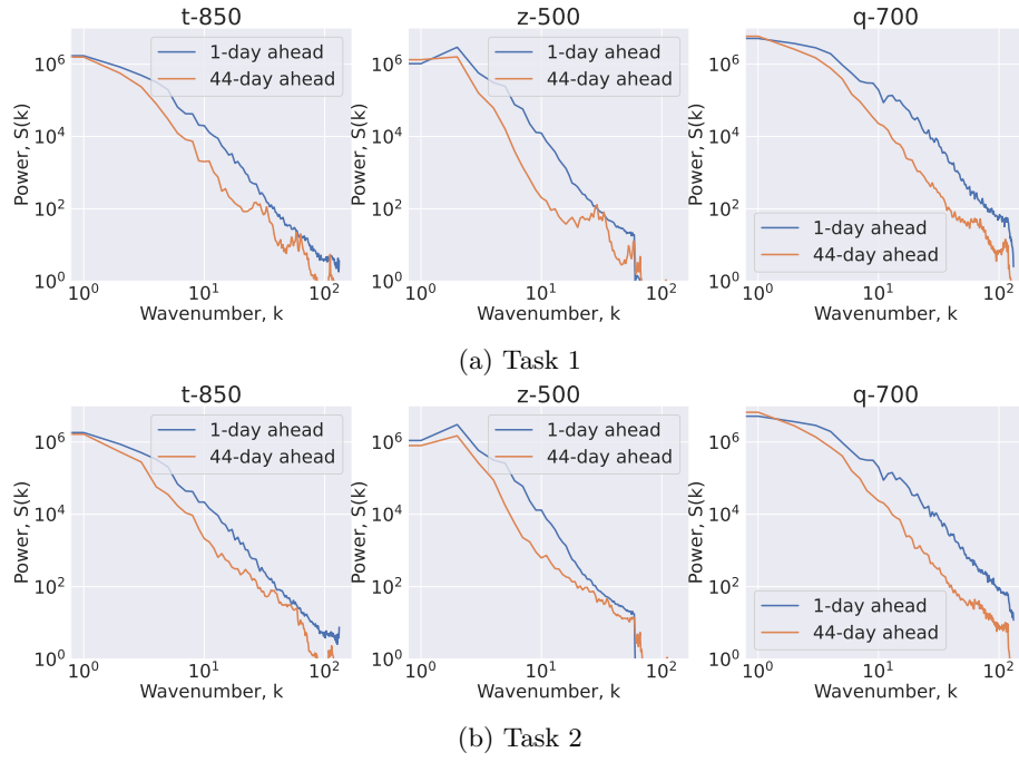
Figure 1: Power spectra for ViT/ClimaX demonstrating decay especially for high k as the lead-time gets larger.
