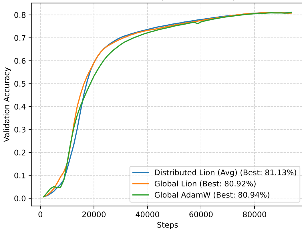
Validation Accuracy Curve on ImageNet
