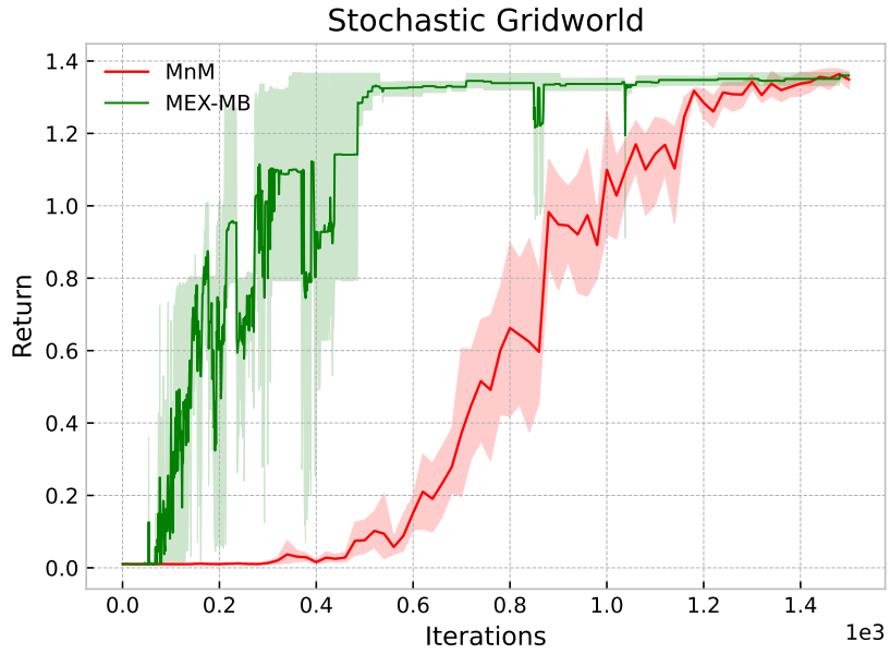
Figure 2: Response to Originality by Reviewer wpG c: Evaluation in the stochastic gridworld environment. The shaded region corresponds to standard deviation using 5 different random seeds.
