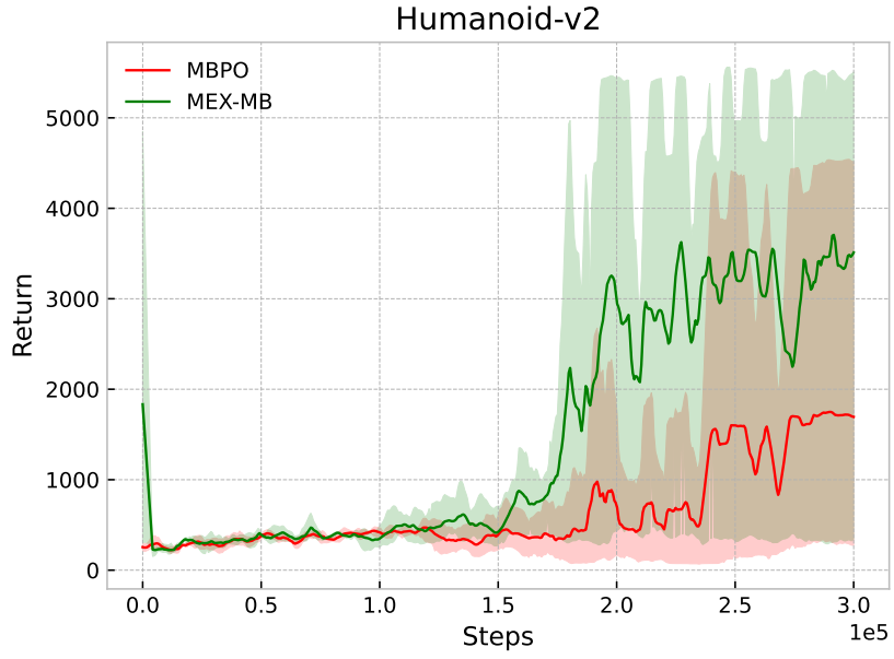
Figure 1: Response to Question 5 by Reviewer vhg d: Evaluation in the humanoid locomotion task. The shaded region corresponds to standard deviation using 5 different random seeds.
