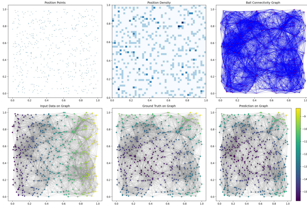
Figure 8: Graph Visualizations for Advection.
