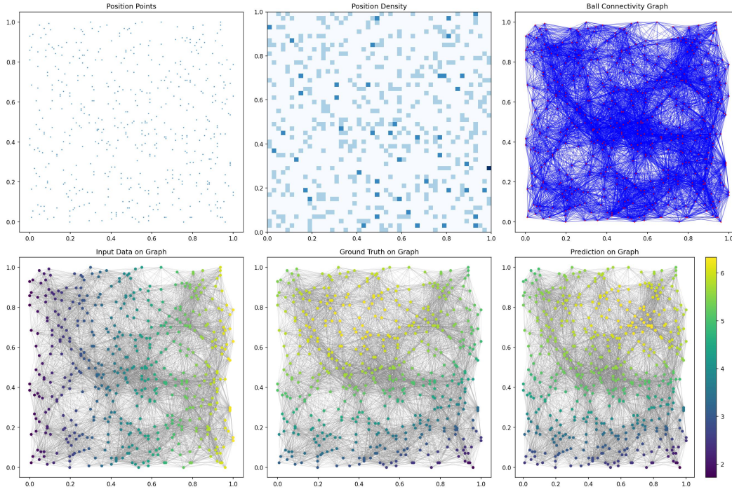
Figure 10: Graph Visualizations for Advection.
