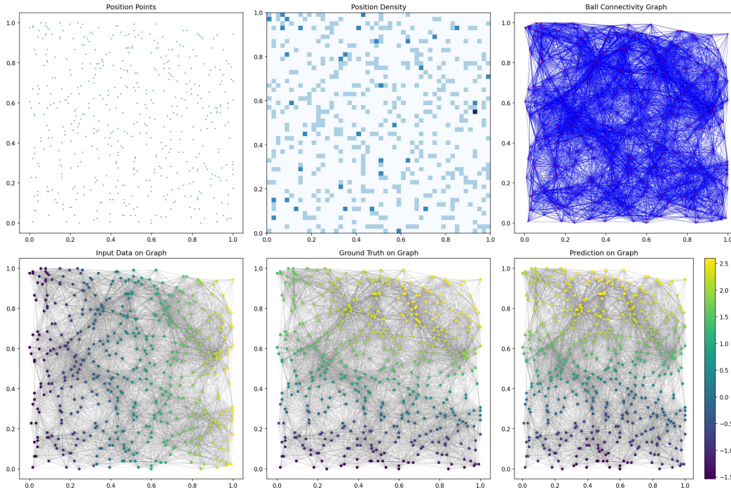
Figure 9: Graph Visualizations for Advection.
