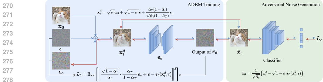
Figure 2: The illustration of ADBM training. The blue block represents the training objective, and the green block represents the extra module for adversarial noise generation. Black arrows denote the computation of L_b , blue arrows denote the computation of L_c used for generating adversarial noise, and red arrows denote the direction of the gradient flow when calculating \epsilon_a .
