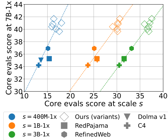
Figure 1: Correlation of architecture scales. Dataset rankings are consistent when training 3B models (green) compared to 7B models (just as they were for 400M and 1B models).
