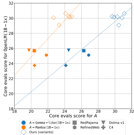
Figure 2: Correlation of architecture variants. Dataset rankings remain consistent when switching from our existing architecture to ones inspired by Gemma and Mamba. Our datasets still perform considerably better than existing baselines.
