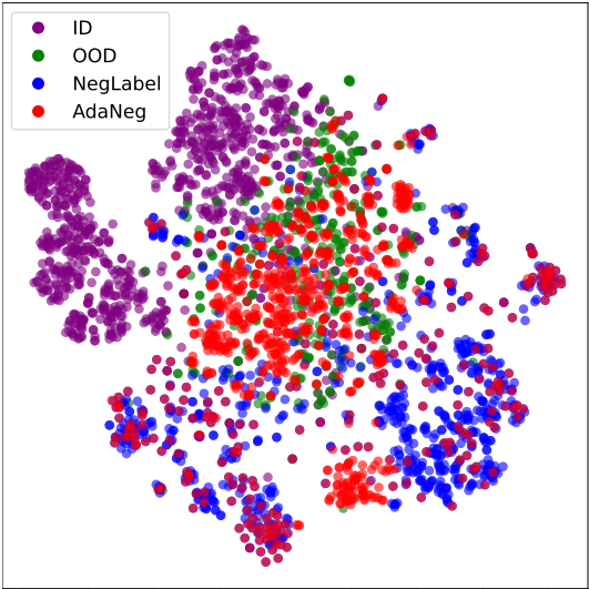
Figure 1: (a) t-SNE Visualization of ID labels, OOD labels, negative labels from NegLabel, and adaptive negative proxies from AdaNeg.
