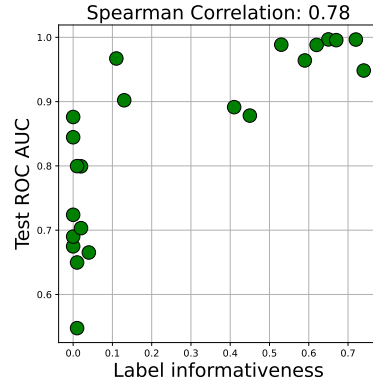
Figure 2: Performance of GraphSAGE on real graphs vs LI_{edge}
