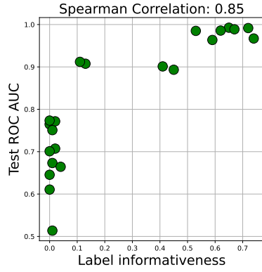
Figure 1: Performance of GAT on real graphs vs LI_{edge}
