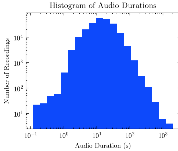
Figure 1: [XHtJ] Dataset summary information
