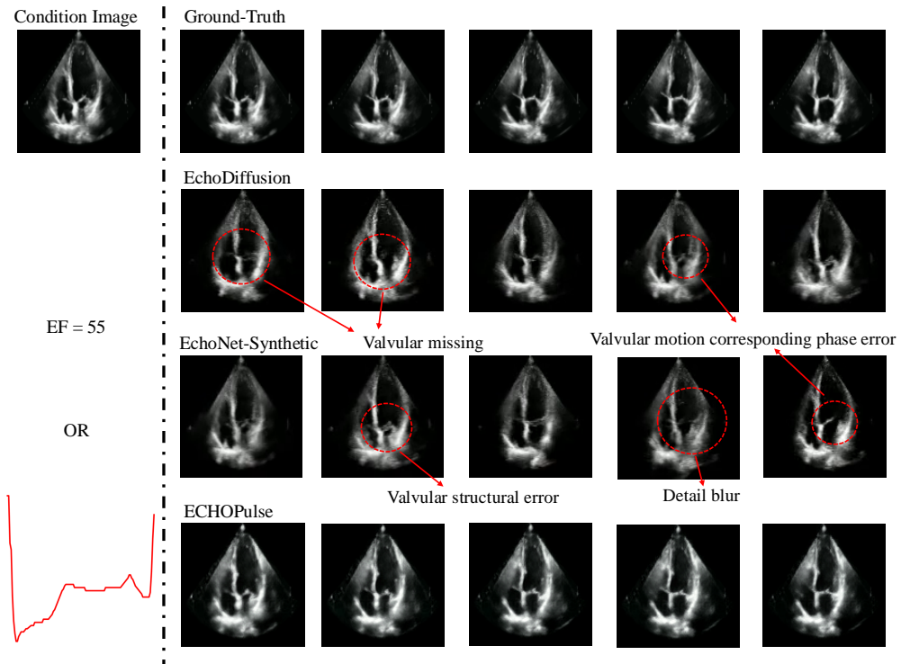
Figure 9: A4C video generation comparison results among ECHOPulse, EchoDiffusion and EchoNet-Synthetic.
