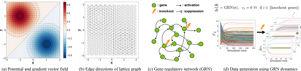
Figure 3: Synthetic datasets. (a-b) Triangular lattice graph with edge directions derived from the gradient of a 2d potential function V (shown in a), creating long-range flows across the graph. (c-d) Gene regulatory network (GRN) represented as a directed graph where nodes are genes and edges denote interactions. Steady-state gene expression levels are obtained from GRN dynamics, with perturbations simulated by setting the expression levels of specific genes to zero.
