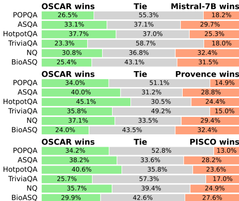
Figure 3: GPT-4 pairwise comparisons. OSCAR-llama, while faster, is on par with no compression baseline, Provence and PISCO.
