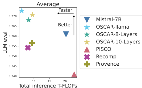
Figure 1: OSCAR models enable faster end-to-end inference with retrieval as well as improved accuracy compared to hard compression methods.
