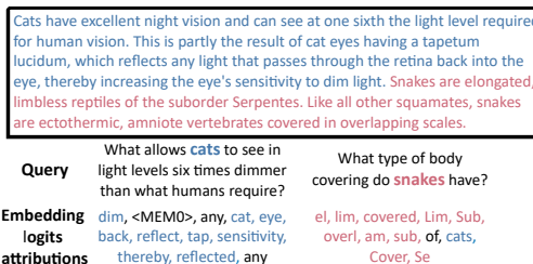
Figure 14: Logits attributions on OSCAR embeddings. Attributed tokens predominantly correspond to an area of the context relevant to the query.
