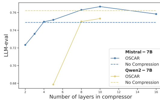
Figure 9: Average accuracy on general domain datasets for OSCAR models where the compressor has a variable number of layers. Performances increase with the number of layers but plateau above 8-10 layers for both Qwen2-7B and Mistral-7B backbones.
