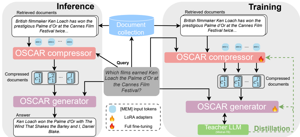
Figure 2: OSCAR overview.
