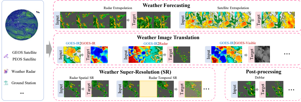
Figure 1: Illustration of the unified representation framework for weather understanding tasks.
