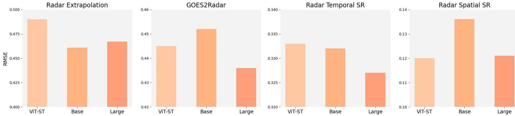
Figure 9: RMSE performance comparison across different model configurations.
