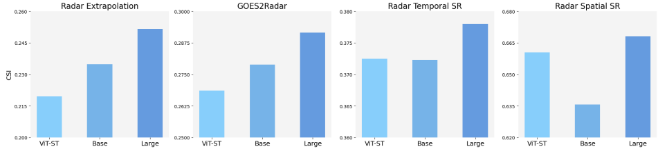
Figure 7: The effect of model sizes. ViT-ST: single-task ViT trained on 0.5 million samples. Base: our WeatherGFM with 100 M parameters trained on 4 million samples. Large: our WeatherGFM with 330 M parameters trained on 4 million samples.
