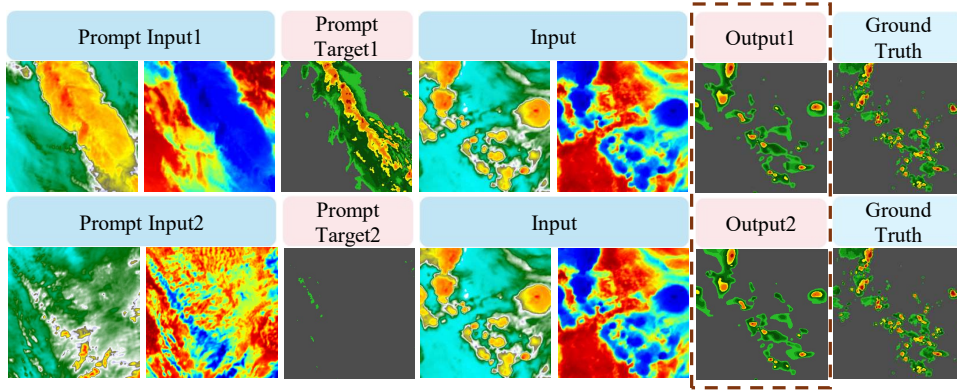
Figure 8: Case studies of our WeatherGFM using different prompts in the GEOS-IR2Radar task.
