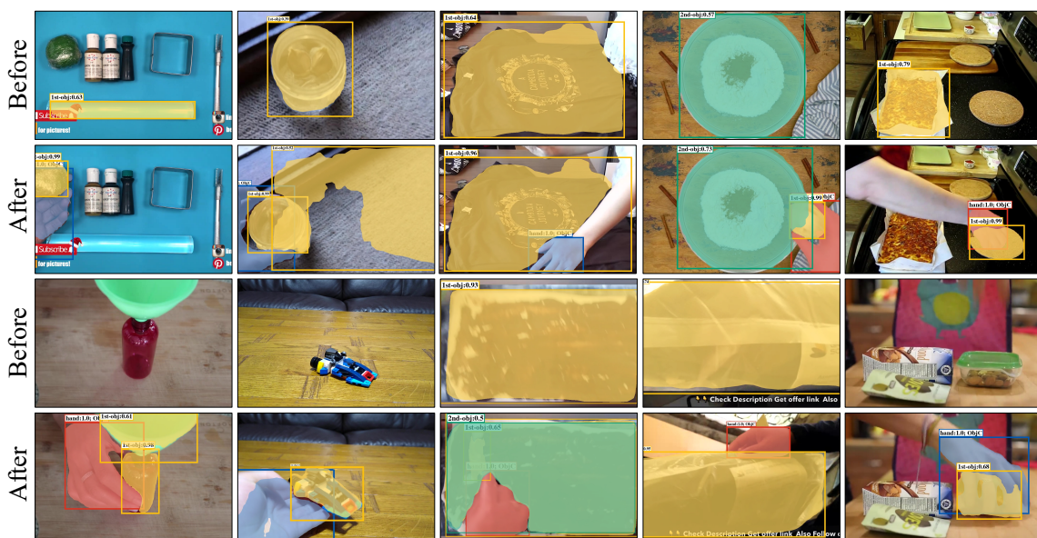
Figure 2: Implicit object relation. Before shows predictions when only objects exist. After shows predictions when hands approach and interact with objects.
