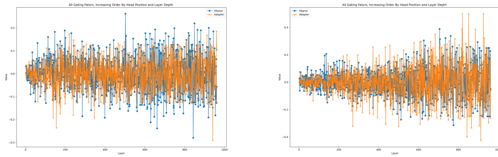
Figure 11: All gating factors in Aligned (Blue) or LLaMA-Adapter Model (Yellow), from first head to last head, and from first adapter layer to last layer. The left are the models trained on Alpaca Dataset, and the right are the models trained on MetaMath Dataset.
