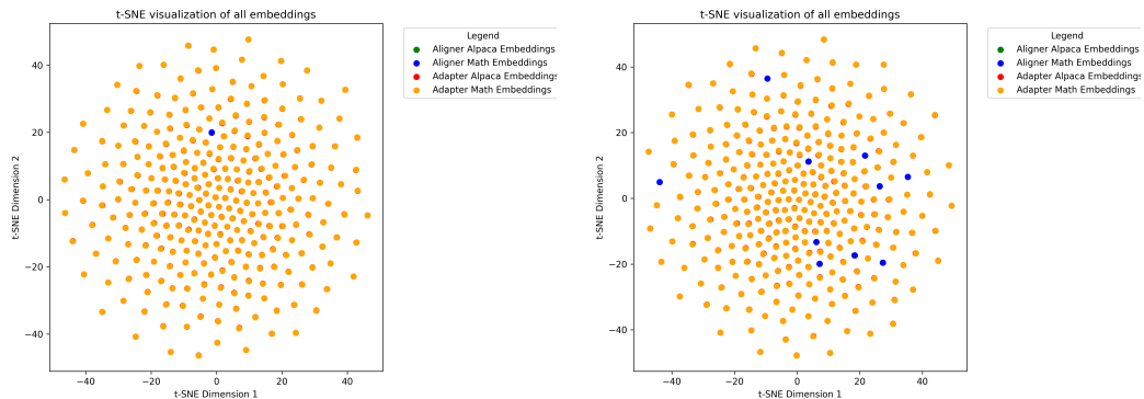
Figure 15: The t-SNE visualization when putting both Aligned and LLaMA-Adapter embeddings trained on both Alpaca and MetaMath dataset (in total 4 different models' embeddings) altogether. The embedding difference between datasets for the same method comparing to the difference between methods for the same dataset is so small that the former one almost completely overlaps with each other.
