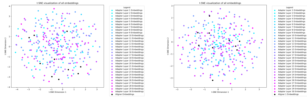
Figure 14: Comparing Aligned *10* Token embedding with tokens of LLaMA-Adapter across all layers using t-SNE method, for both the ones trained on Alpaca Dataset (Left) and the ones trained on MetaMath Dataset (Right). The black dots are the Aligned embedding, while the rest are the LLaMA-Adapter embeddings.
