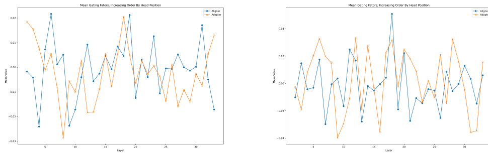
Figure 10: The mean value of gating factors based on attention head position across layers in Aligned (Blue) or LLaMA-Adapter Model (Yellow). The left are the models trained on Alpaca Dataset, and the right are the models trained on MetaMath Dataset.
