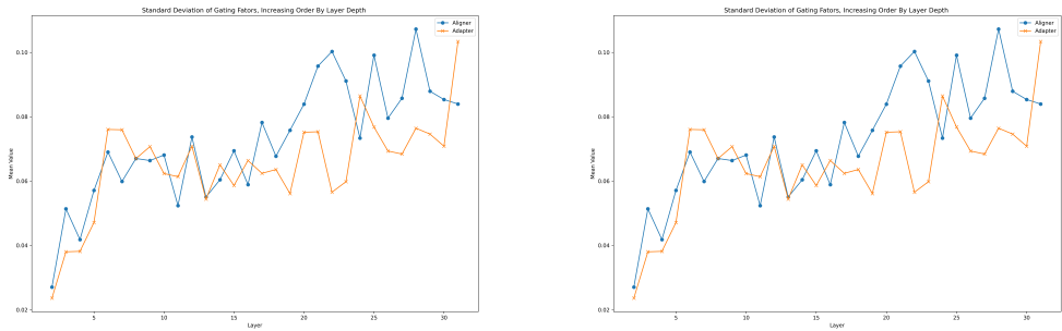
Figure 7: The standard deviation of gating factors for a layer in Aligner (Blue) or LLaMA-Adapter Model (Yellow). The left are the models trained on Alpaca Dataset, and the right are the models trained on MetaMath Dataset.
