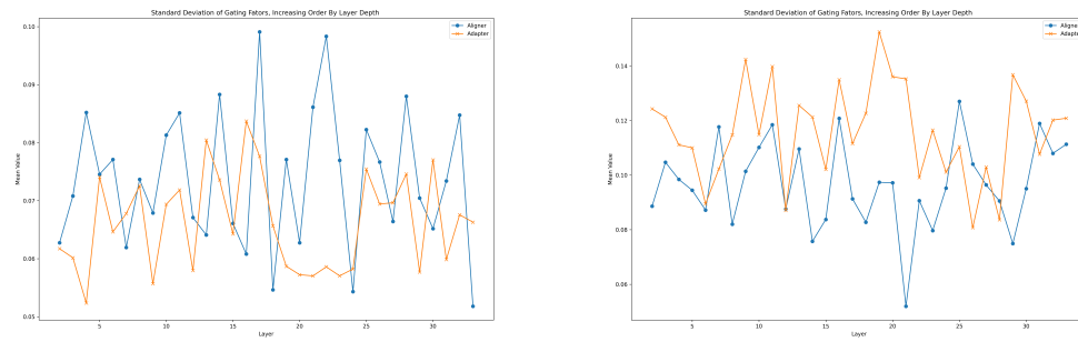
Figure 9: The standard deviation of gating factors based on attention head position across layers in Aligned (Blue) or LLaMA-Adapter Model (Yellow). The left are the models trained on Alpaca Dataset, and the right are the models trained on MetaMath Dataset.
