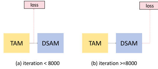
Figure 1: The details of the two training phases.
