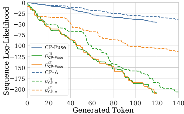
Figure 6: (Same as Figure 2) Log-likelihood for the sequence produced by CP-Fuse and CP- \Delta , and the corresponding base models p^{(1)} and p^{(2)} at each token in greedy decoding. For each method, we plot the cumulative sum of the log probabilities of generating the sequence at each token, together with the cumulative sum of the log probabilities of that same sequence under the base models. Due to the balancing property, CP-Fuse achieves \log p^{(1)}(y_{\leq t}|x) \approx \log p^{(2)}(y_{\leq t}|x) at all steps of the generation, indicating that the tokens produced by CP-Fuse are roughly equally likely under both base models, hence preventing the reproduction of memorized samples. In contrast, CP- \Delta places significantly more weight on the second model p^{(2)} , as evidenced by the much higher log-likelihood of the generated tokens under p^{(2)} compared to p^{(1)} .
